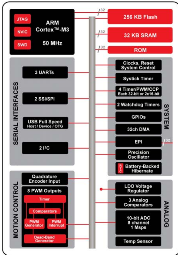
LM3S3000 Series Block Diagram. This block diagram shows the superset of features for the LM3S3000 series of microcontrollers.
