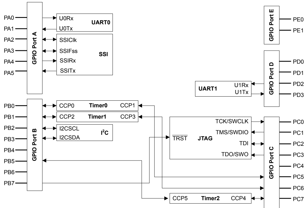
Figure 8-1. GPIO Module Block Diagram
