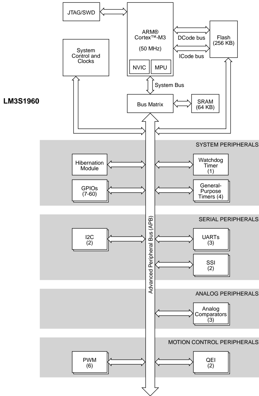
Figure 1-1. Stellaris® LM3S1960 Microcontroller High-Level Block Diagram
