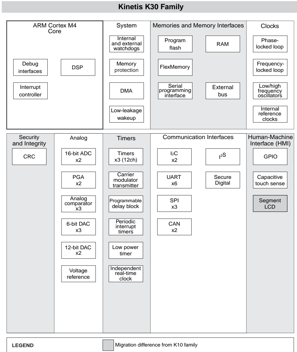
Figure 3. K30 Block Diagram
