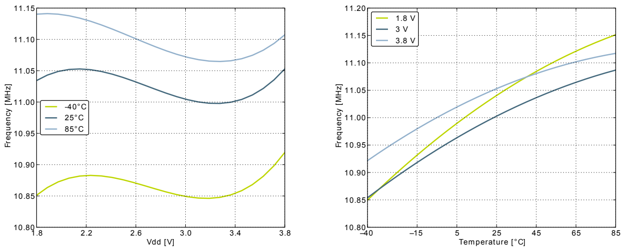
Figure 3.11. Calibrated HFRCO 14 MHz Band Frequency vs Supply Voltage and Temperature
