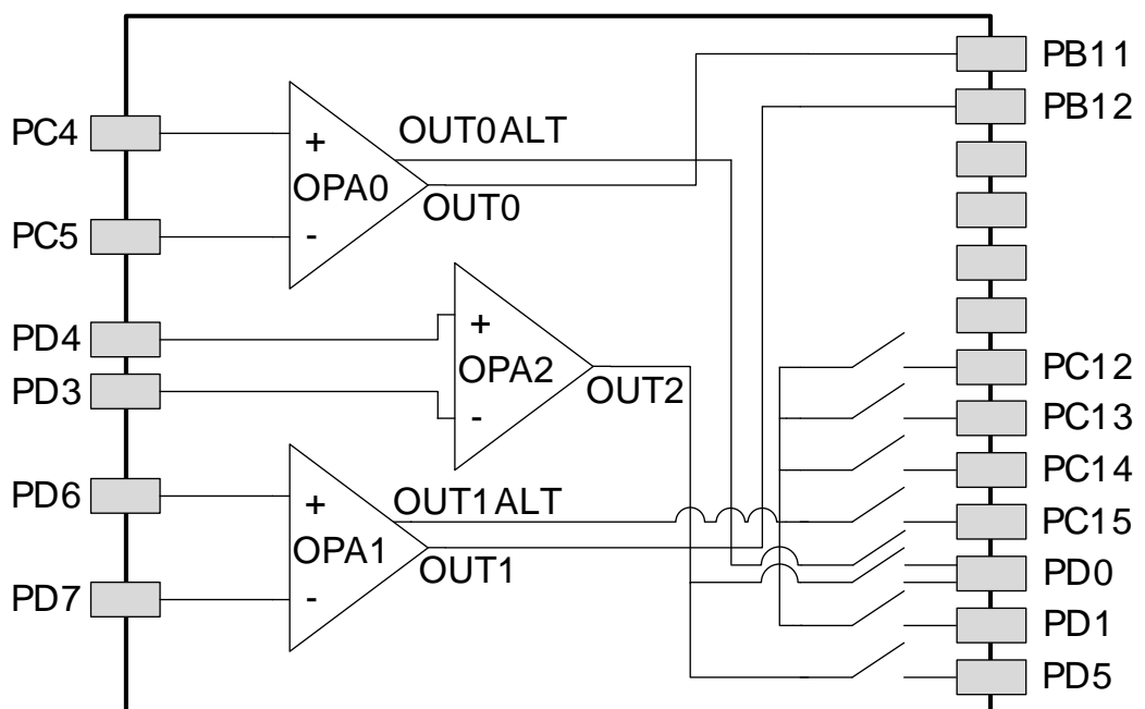
Figure 4.2. Opamp Pinout
