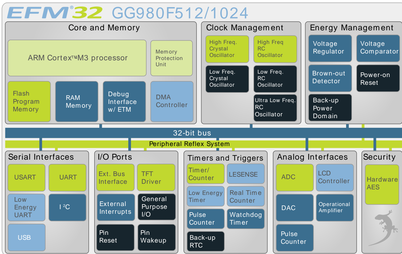
Figure 2.1. Block Diagram
