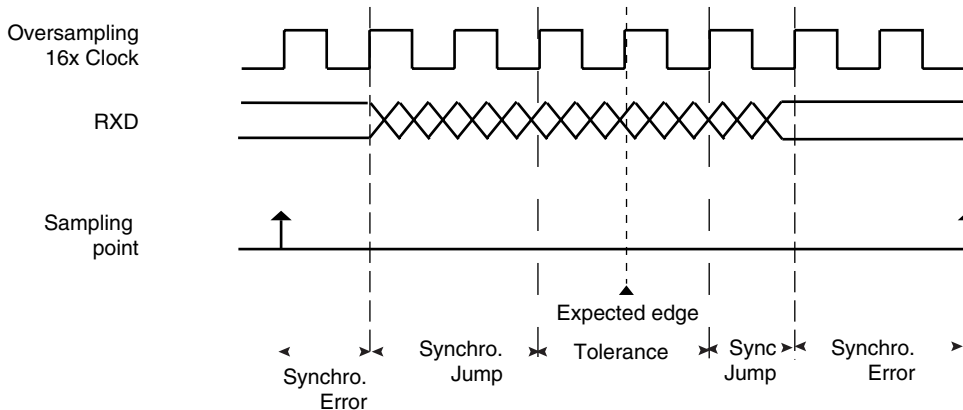
Figure 29-11. Bit Resynchronization
