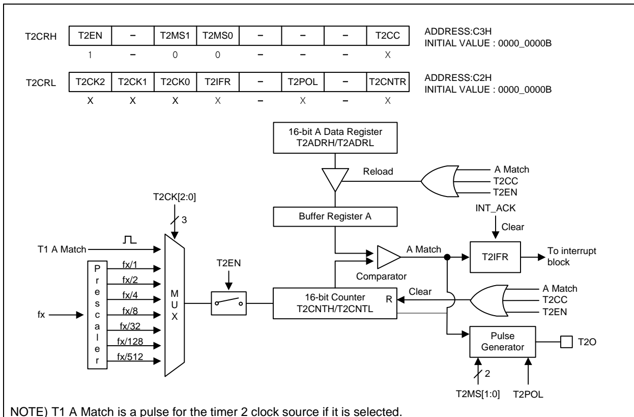
Figure 11.22 16-Bit Timer/Counter Mode for Timer 2
