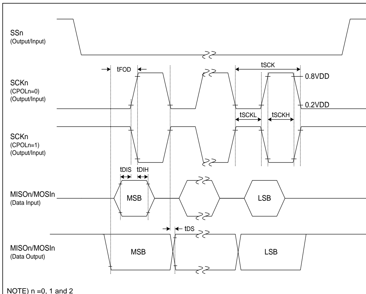
Figure 7.2 SPI0/1/2 Timing
