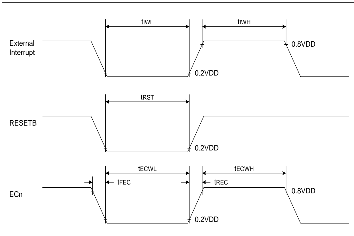
Figure 7.1 AC Timing
