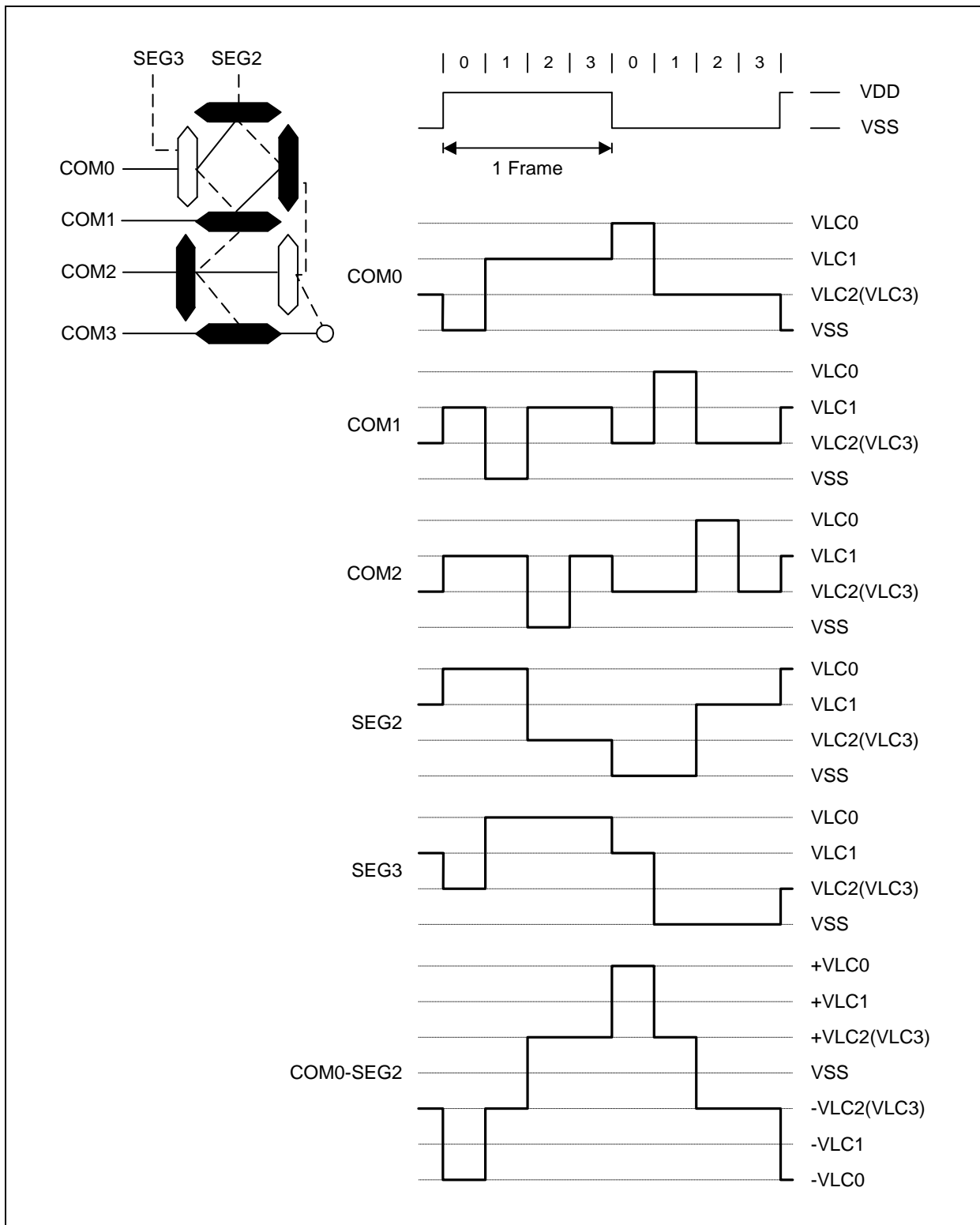
Figure 11.102 LCD Signal Waveforms (1/4Duty, 1/3Bias)
