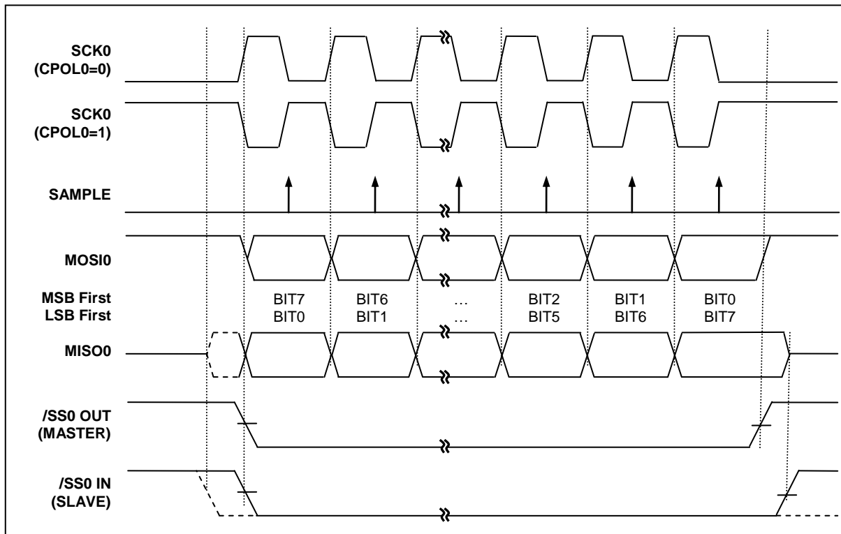
Figure 11.65 USIO SPI Clock Formats when CPHA0=1
