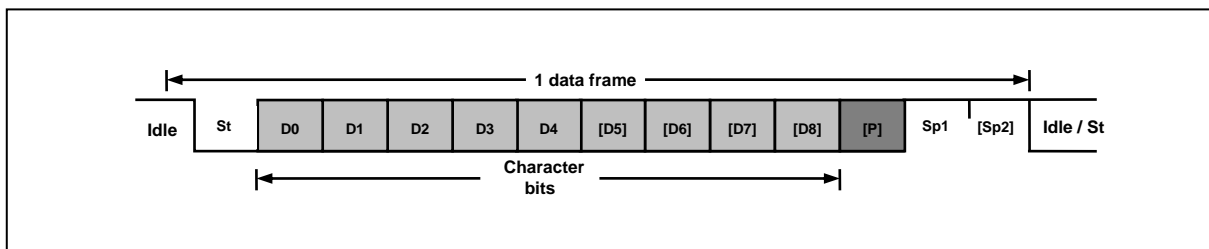
Figure 11.81 Frame Format (US11)
