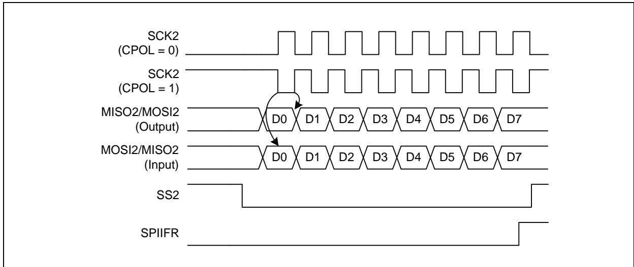
Figure 11.50 SPI 2 Transmit/Receive Timing Diagram at CPHA = 0
