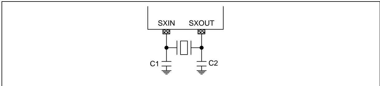
Figure 7.10 Crystal Oscillator
