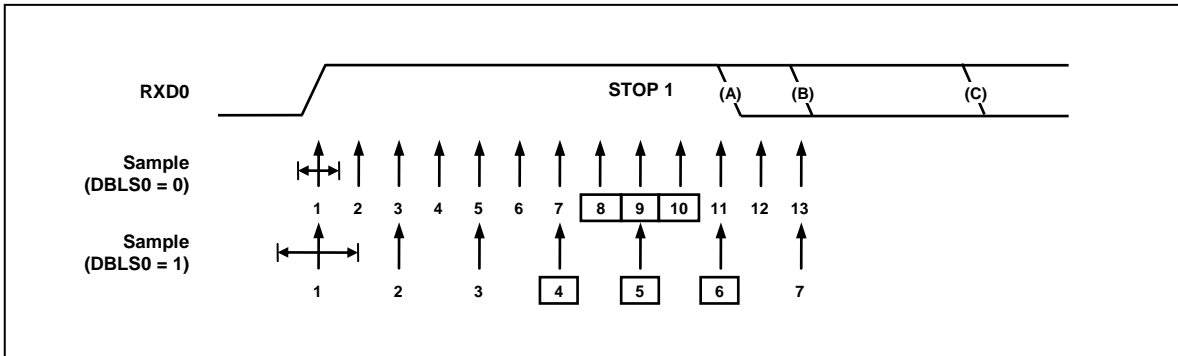
Figure 11.63 Stop Bit Sampling and Next Start Bit Sampling (US10)
