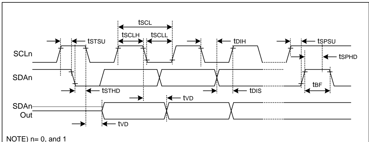
Figure 7.5 I2C0/1 Timing
